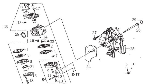
Carburetor
