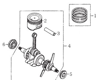
Crankshaft/Piston
