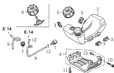
Fuel tank
