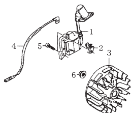
Flywheel
