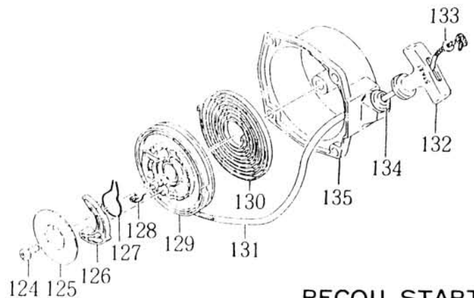
RECOIL STARTER
