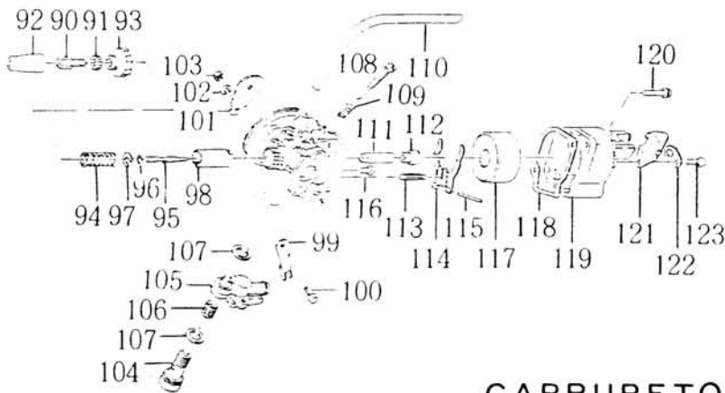
CARBURETOR
